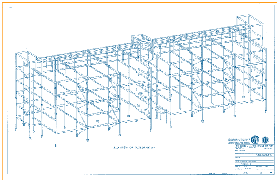
Building 7, whose 3-D erection drawing is shown here, was erected in three weeks.
