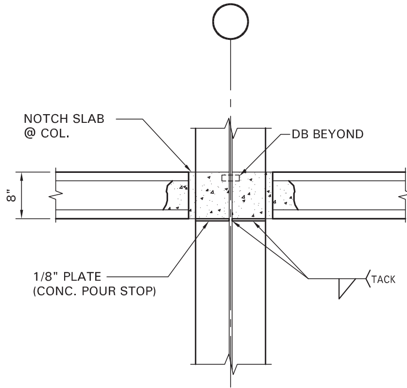
TYPICAL SECTION THRU WF COLUMN AT GROUT POUR STOP
